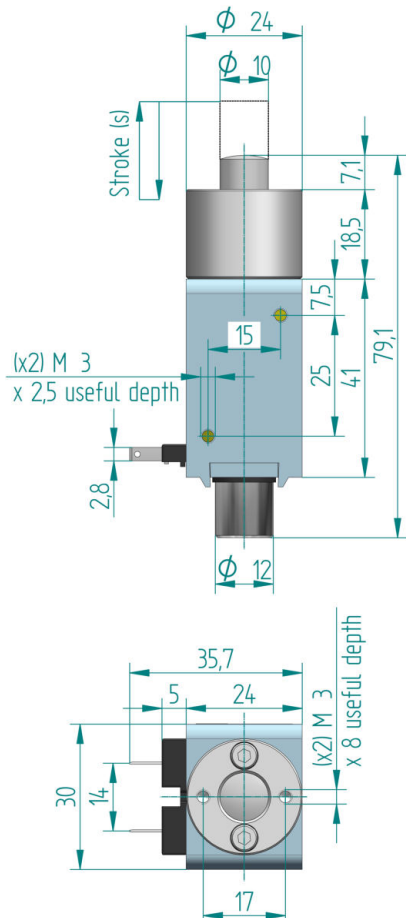
Solenoid without voltage
